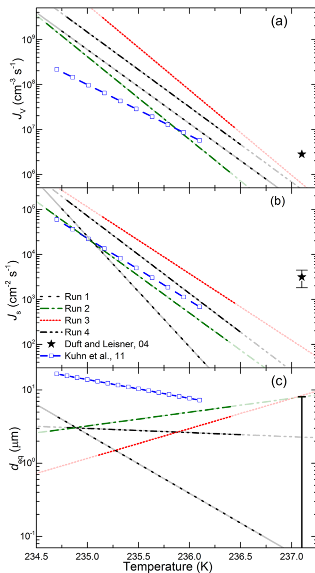
Figure 7. Volume (a) and surface (b) nucleation rate coefficients resulting from combined surface and volume nucleation fits (see Table 2). (c) d_{eq}(T) , the diameter at which surface and volume freezing are equivalent (eq 6). For comparison, the parametrization of Kuhn et al. 15 and limiting data from Duft and Leisner 14 are shown. The data from Duft and Leisner 14 corresponds to 100% of freezing due to the volume (panel a) or surface (panel b). For surface nucleation the data vary by a factor of 2.5, the range of which is given by error bars, for volume nucleation the range is smaller than the data point. At 237.1 K all of the experiments give a calculated d_{eq}(T) less than the \sim 8 \mu\text{m} limit from Duft and Leisner, 14 which is shown as a single error bar in panel c. The data are extrapolated beyond experimental temperature ranges, with temperatures outside this range denoted by fainter lines.
