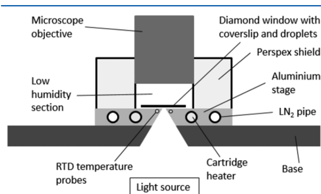
Figure 1. Schematic of the cold stage. The cold stage itself consists of a small aluminum block with heaters, liquid nitrogen pipes ( \text{LN}_2 ), and temperature probes embedded into it. The droplet containing coverslip is placed on a diamond window, which bridges the hole in the stage that provides light for transmission microscopy. See section 2 for further details.
