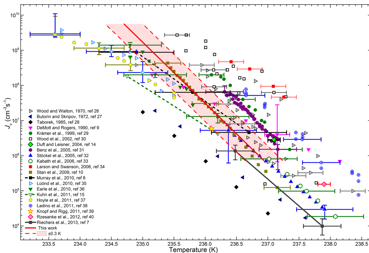
Figure 4. New volume based nucleation rates in comparison with the literature data. 7–10,14,15,26–40 For clarity, only a few sample error bars are provided for each data set.
