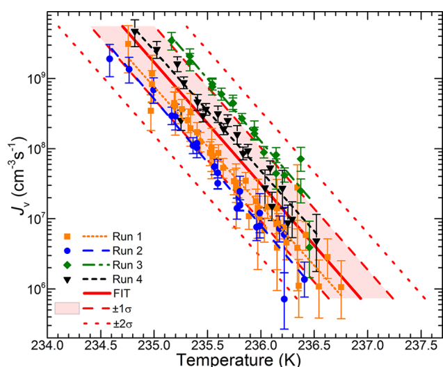
Figure 3. Experimental homogeneous volume nucleation rate coefficients from four experiments with a cooling rate of 1 \text{ K min}^{-1} . The overall fit is shown in red ( \ln(J_V(T)) = -4.0106T + 963.706 ), with a shaded area and dashed lines giving the 1\sigma standard deviation and dotted lines for the 2\sigma range. For each experiment a fit to eq 2 has been performed ( Table 1 ). The fitting process was by a least sum of squares, weighted by the uncertainty in the nucleation rate (see Supporting Information ). The fit gives an R^2 value of 0.947.
