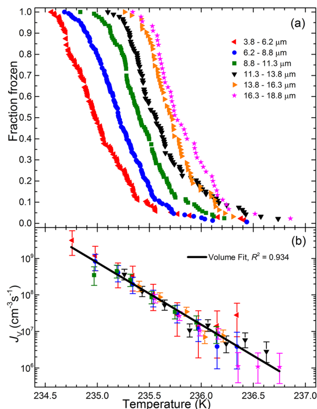
Figure 2. (a) Sample frozen fraction curves for Run 1. (b) Volume nucleation rate coefficients calculated for the freezing shown in panel (a). The frozen fraction of a size bin is defined as the cumulative number of frozen droplets divided by the starting number of droplets. A fit to the nucleation rate coefficients is provided ( \ln(J_v(T)) = -3.9126T + 939.916 , R^2 = 0.934 , see Table 1 for fits to the other runs). Quoted droplet sizes are the diameters of the sessile droplets on the surface. Note that the higher time resolution of the freezing data in panel (a) can result in several freezing observations being grouped into each \Delta t period in panel (b).
