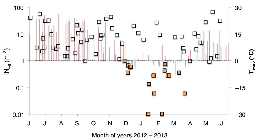
Fig. 6. Time course of IN_{-8} at Chaumont (symbols) and maximum daily temperature (columns). Full symbols indicate cold days ( T_{\max} < 0^\circ\text{C} ). Values of IN_{-8} below detection limit are set to 0.01 \text{ m}^{-3} .
