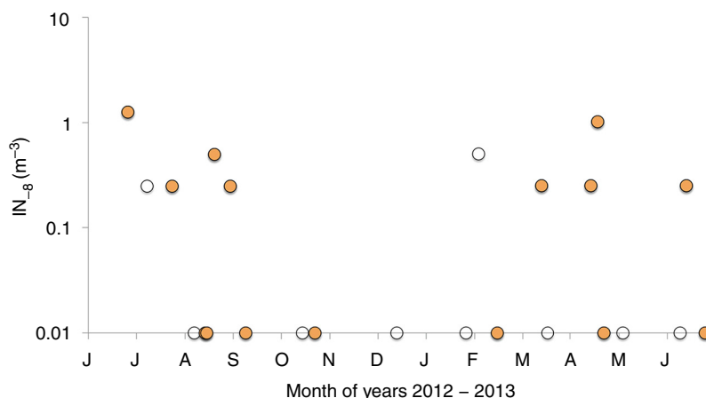
Fig. 3. Time course of IN_{-8} at Izaña (full symbols indicate Sahara dust events). Values of IN_{-8} below detection limit are set to 0.01 \text{ m}^{-3} .
